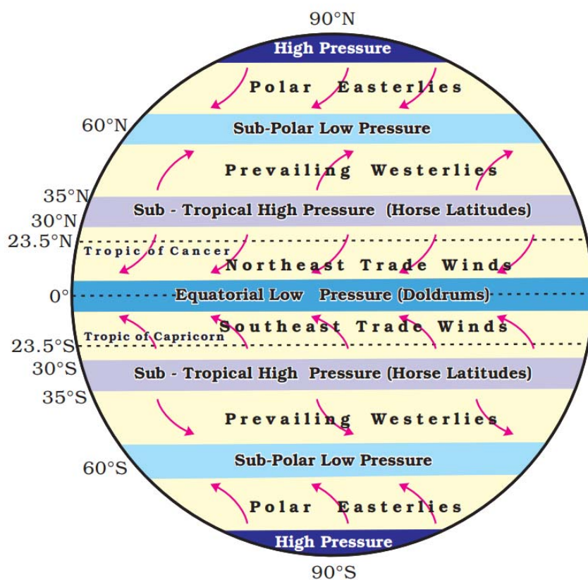
4.4: Major Pressure Belts and Wind System
